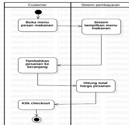
Figure 4. Food Ordering Activity Diagram
