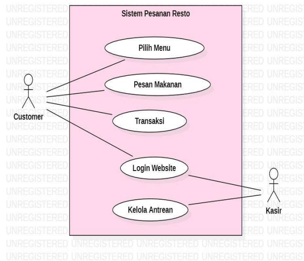
Figure 2. Mavera Use Case Diagram
