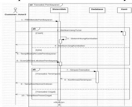
Figure 10. Payment Transaction Sequence Diagram
