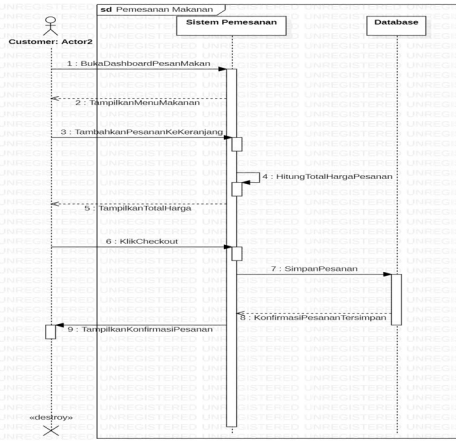
Figure 9. Food Ordering Sequence Diagram
