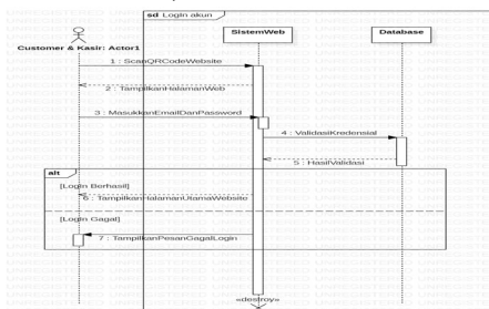
Figure 8. Account Log In Sequence Diagram
